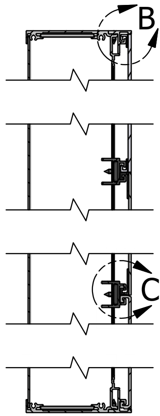
CABINET SECTION-VIEW THRU HORIZONTALS
